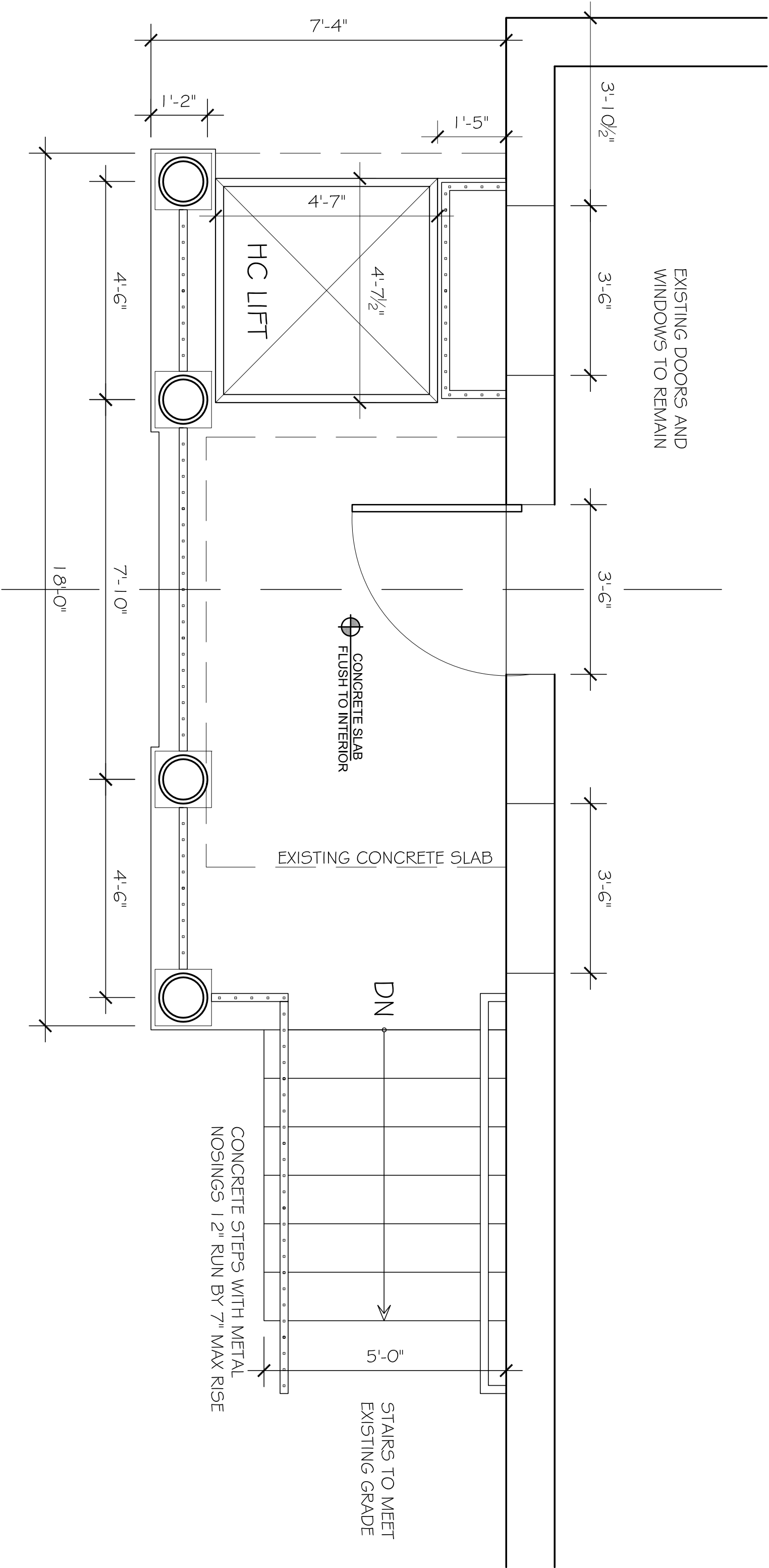
PROPOSED PORTICO PLAN 1/2" = 1'-0"
